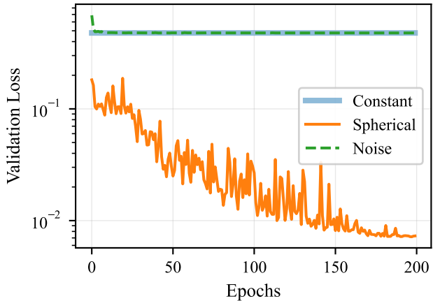
SE(3)-Transformer Backbone
