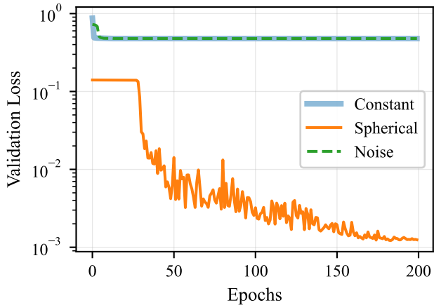
GATr Backbone
